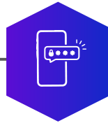
Code Verification
